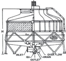
AFT 400-1500
